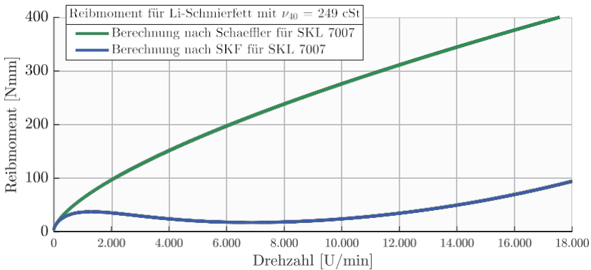
Fig. 1: Friction torque calculated using the catalog method according to Schaeffler Eq. (1) and SKF Eq. (2) for the angular contact ball bearing 7007 and a Li grease with a base oil viscosity of 249 mm 2 /s at 40 °C
